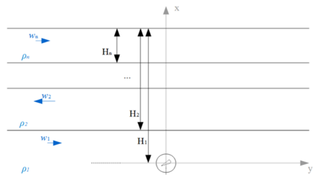
Fig. 2. Stratified continuous medium figure.
