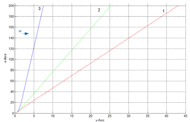
Fig. 4. Motion trajectories of the submarine craft in accordance with system (3).
